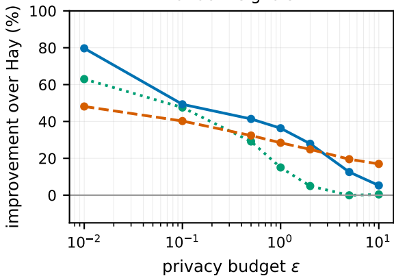
random signals
