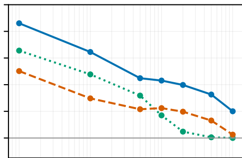
sparse signals
