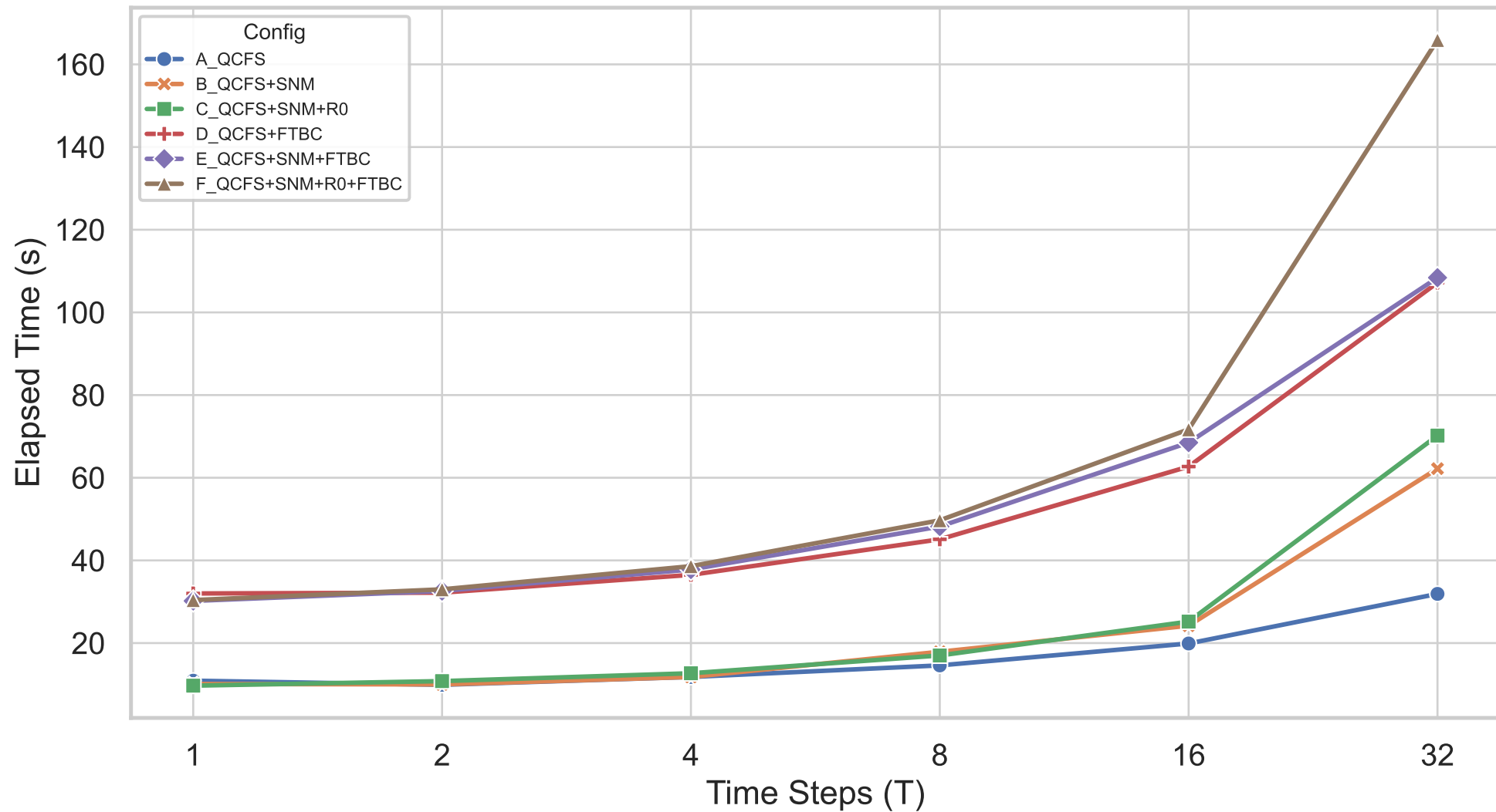
Ablation Study on CIFAR-100 / VGG16 (Elapsed Time)
