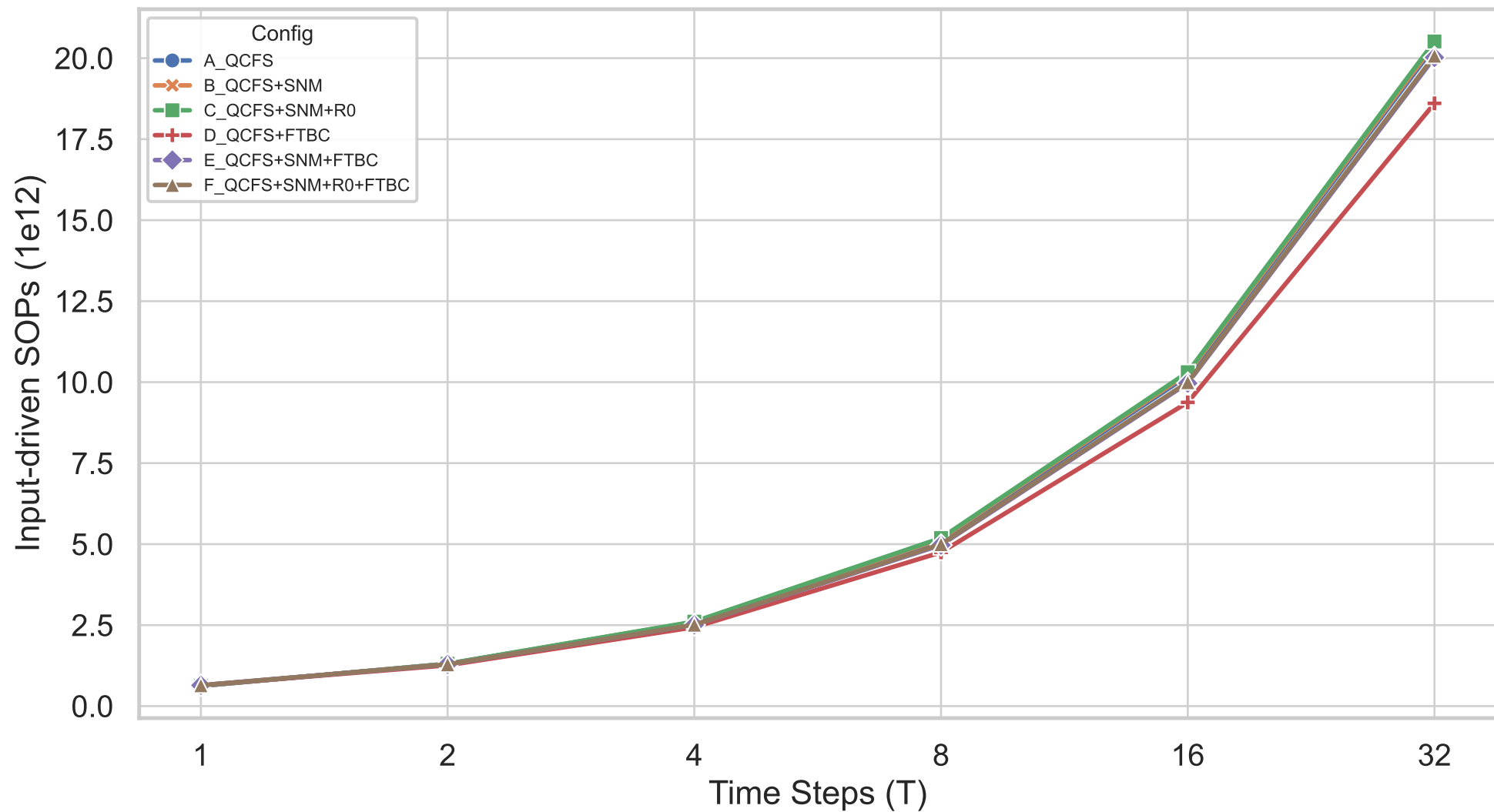
Ablation Study on CIFAR-100 / VGG16 (Input-driven SOPs)
