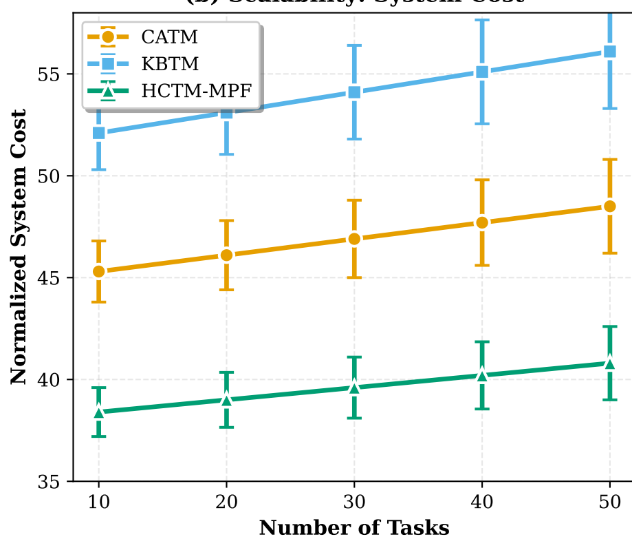
(b) Scalability: System Cost
