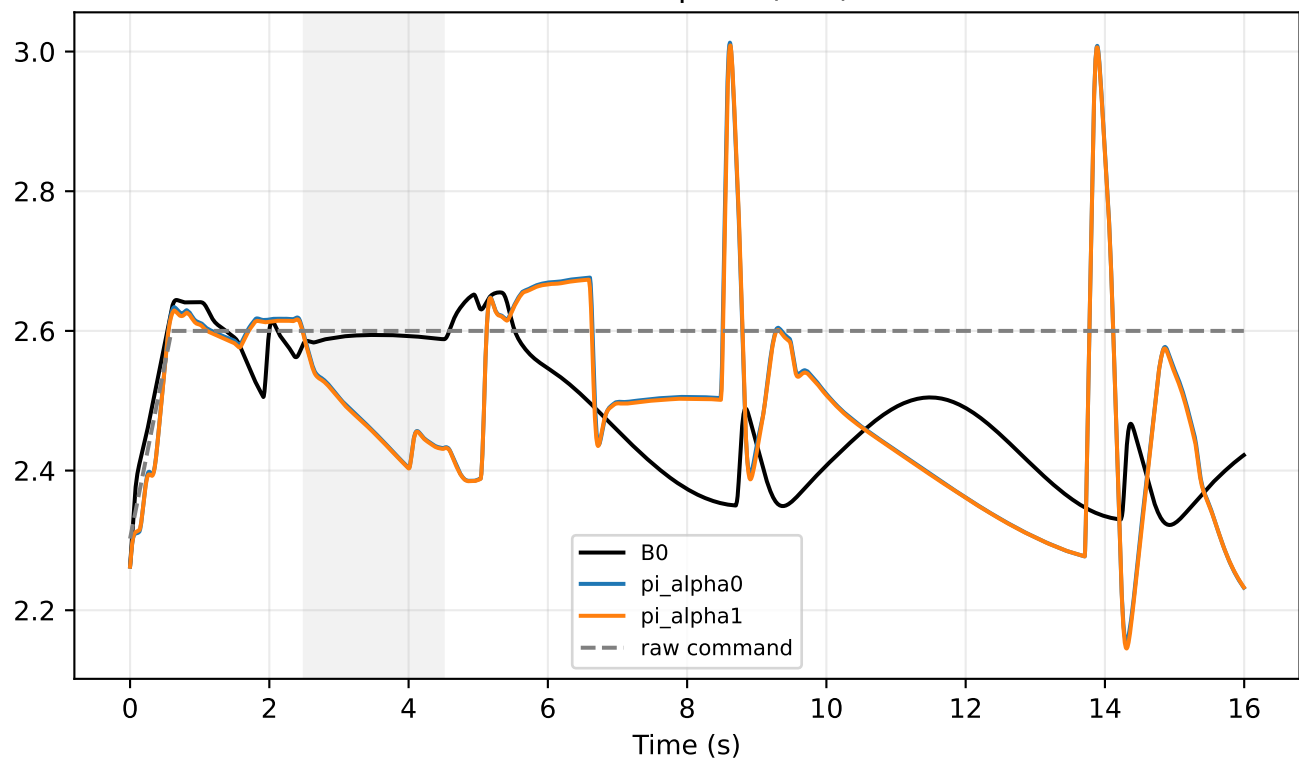
Roll (rad)
