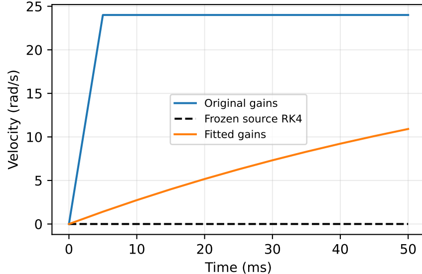
rearwheel_joint input=24, initial qd=0
