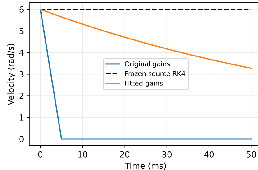
rearwheel_joint input=0, initial qd=6
