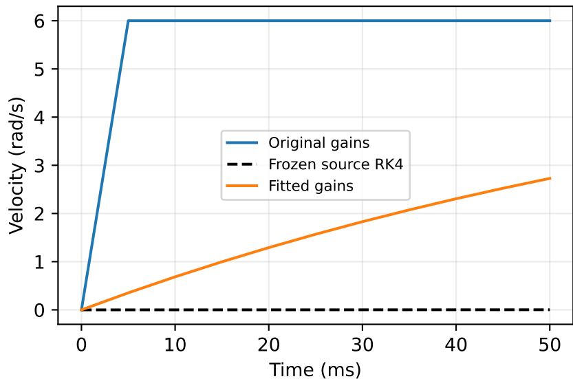
rearwheel_joint input=6, initial qd=0
