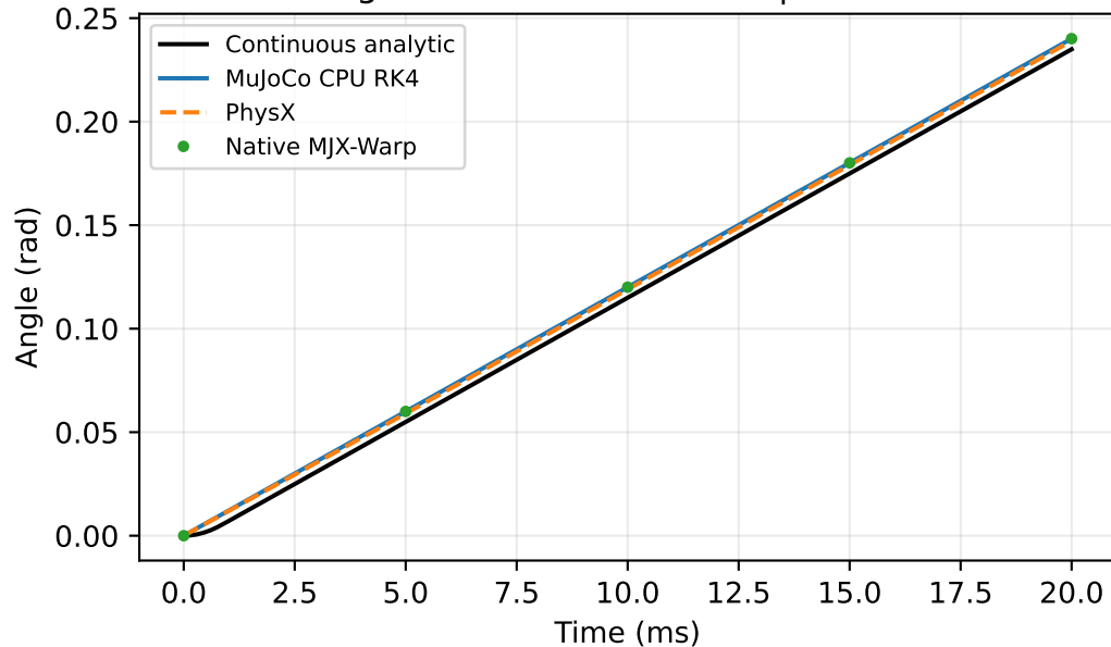
Original isolated rear rotor | dt=5 ms
