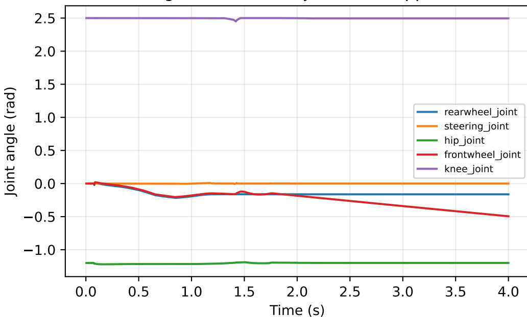
Angles (continuous joints unwrapped)
