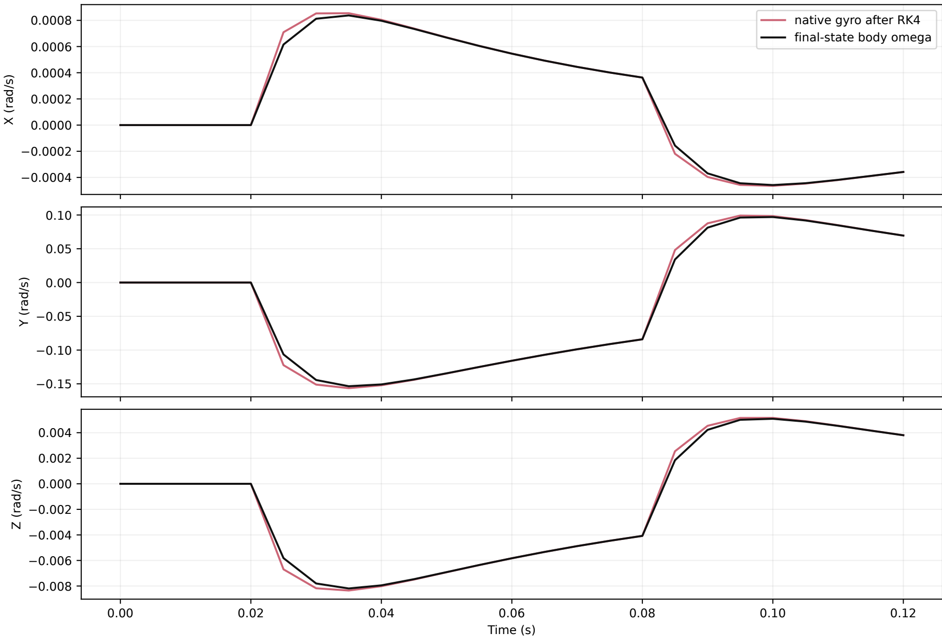
knee_pulse | actual MJX-Warp sensor vs final state
