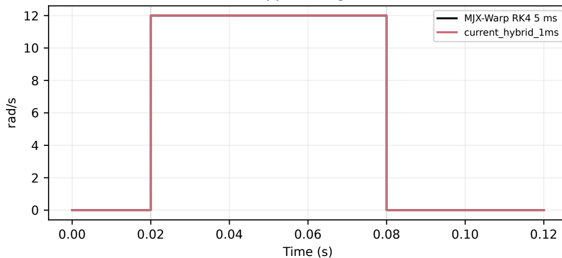
End-state joint velocity
