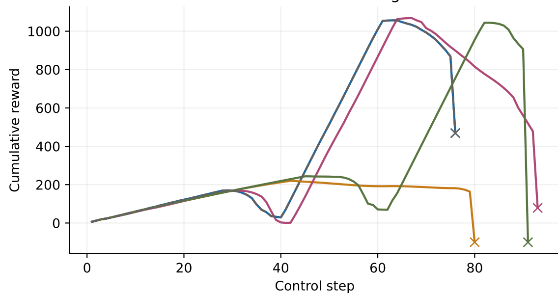
Cumulative reward including failure
