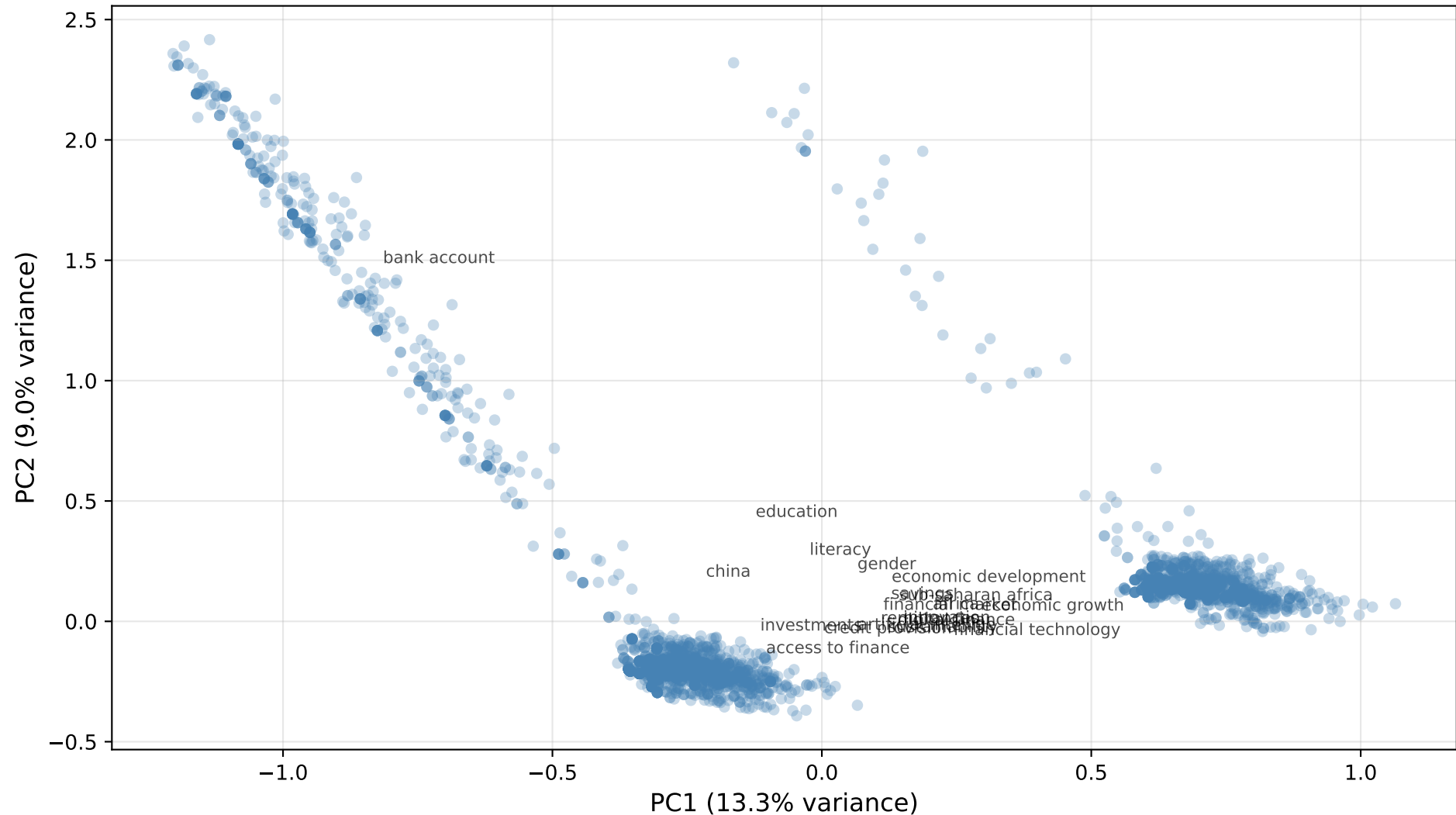
Multiple Correspondence Analysis Map (PCA-based)
