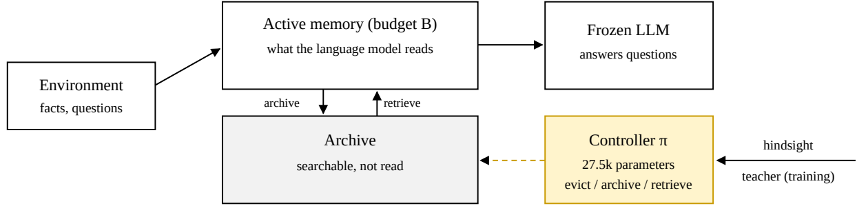
Figure 1. The controller decides what the frozen language model sees. During training only, a hindsight teacher labels its decisions.
