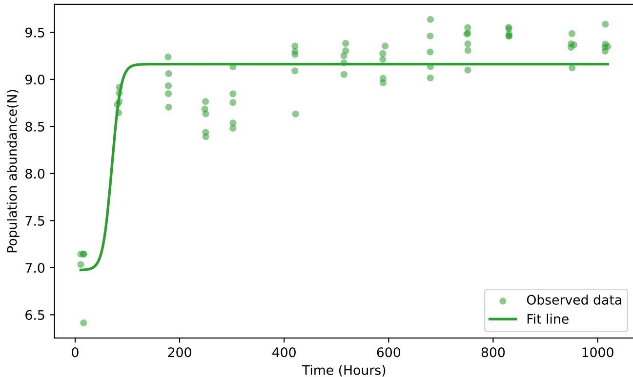
Baranyi model fit at 25 °C
