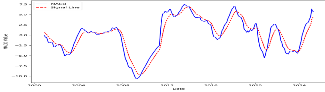
C MACD Analysis
