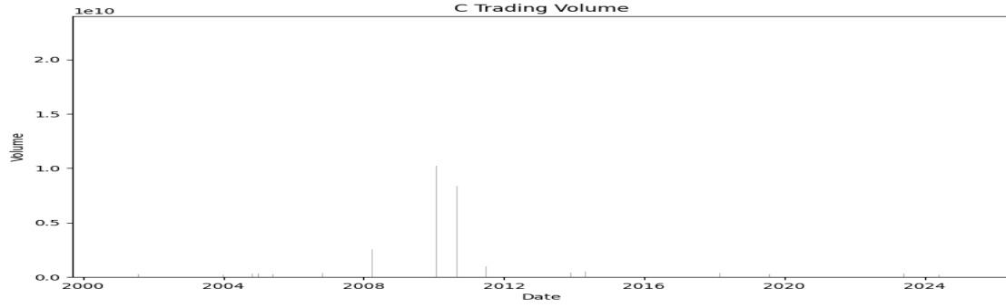
C Trading Volume
