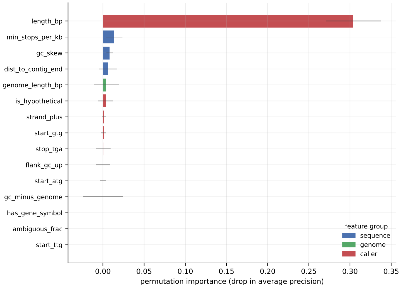
What the forest used, measured on held-out genomes
