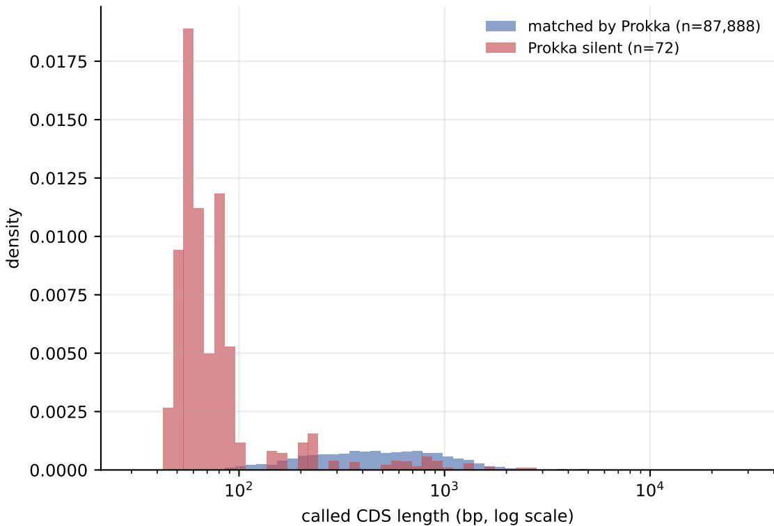
Length of Bakta calls, by whether Prokka agreed
