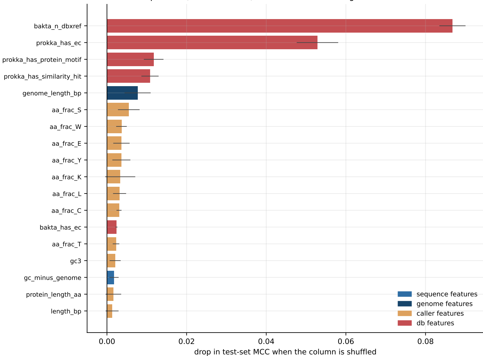
Permutation importance, random forest, measured on held-out genomes
