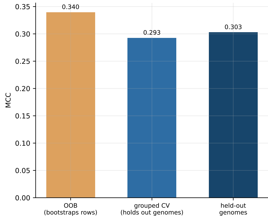
Genome-level leakage: OOB exceeds grouped CV by +0.047
