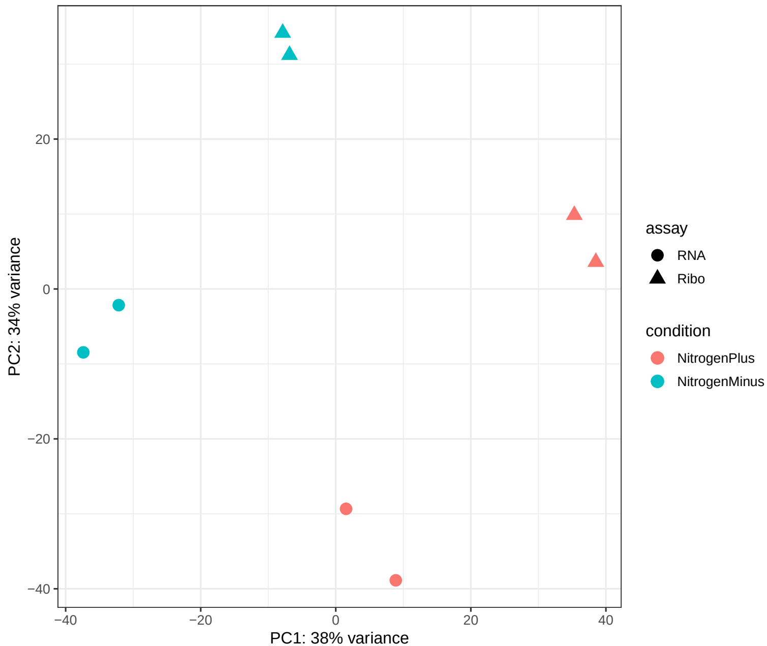
PCA of VST-transformed counts
