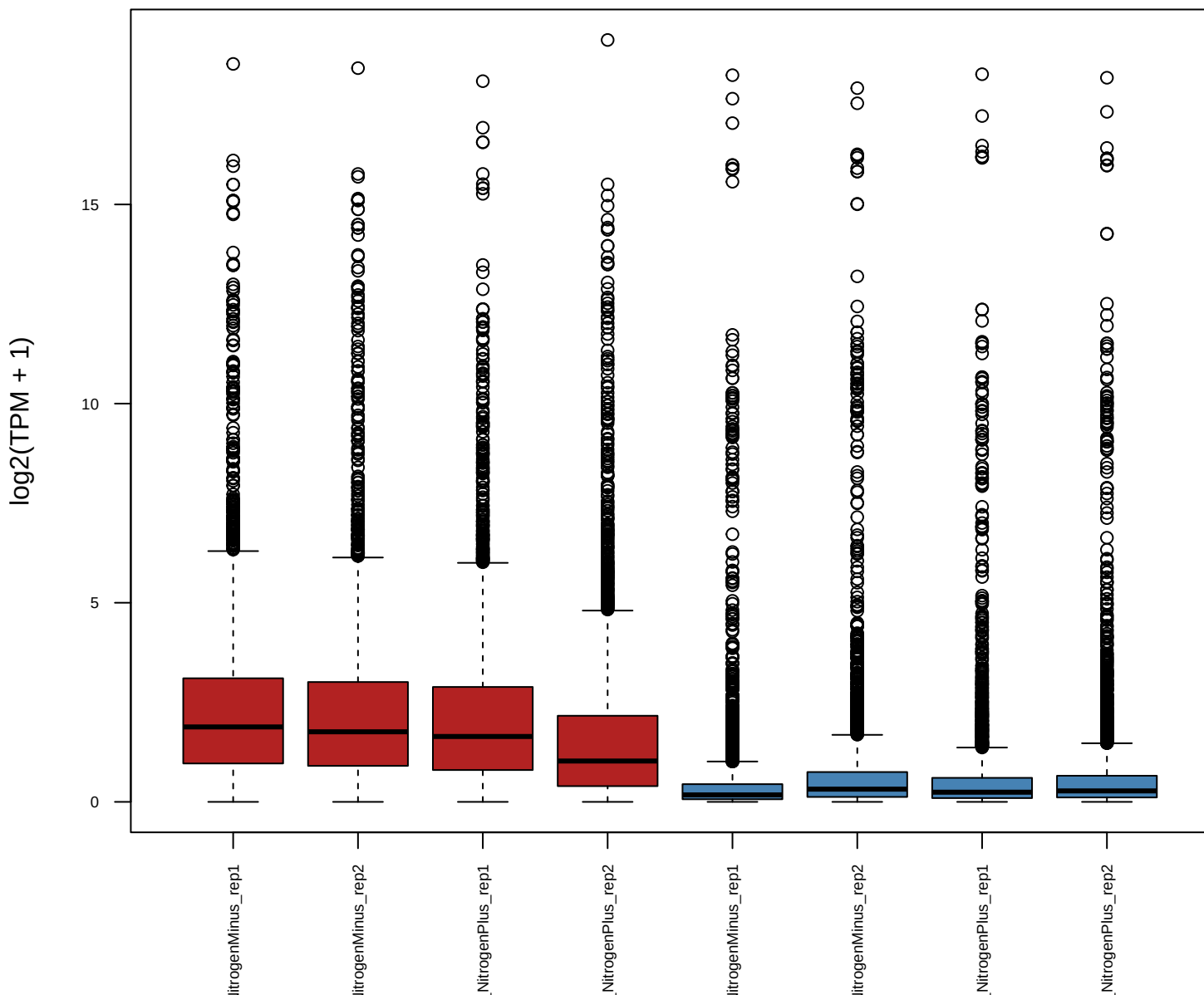
TPM distribution per library
