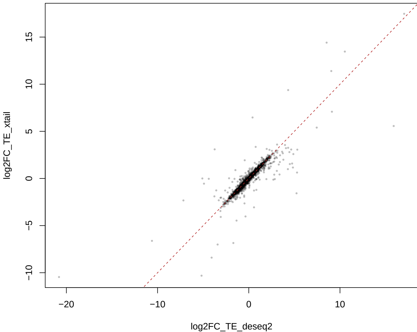
deseq2 vs xtail ( r = 0.897 )
