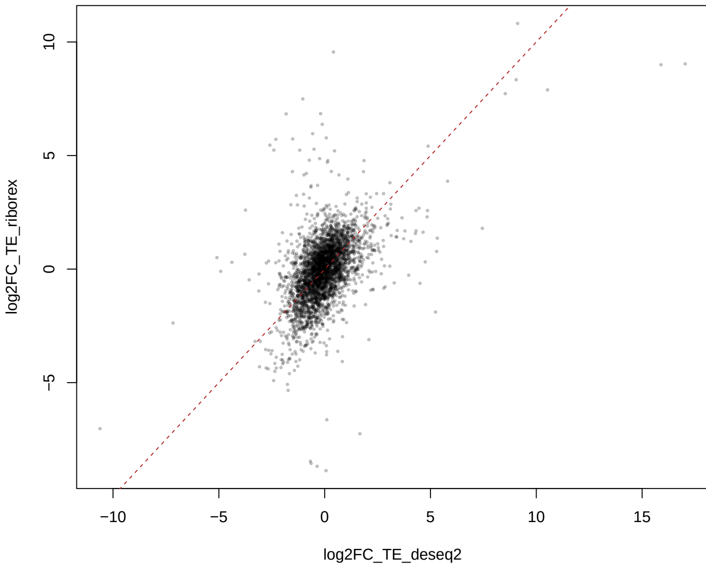
deseq2 vs riborex ( r = 0.502 )
