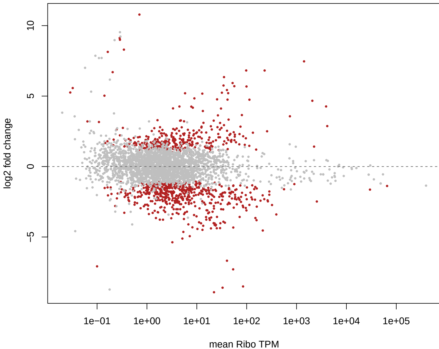
Ribo log2FC vs expression
