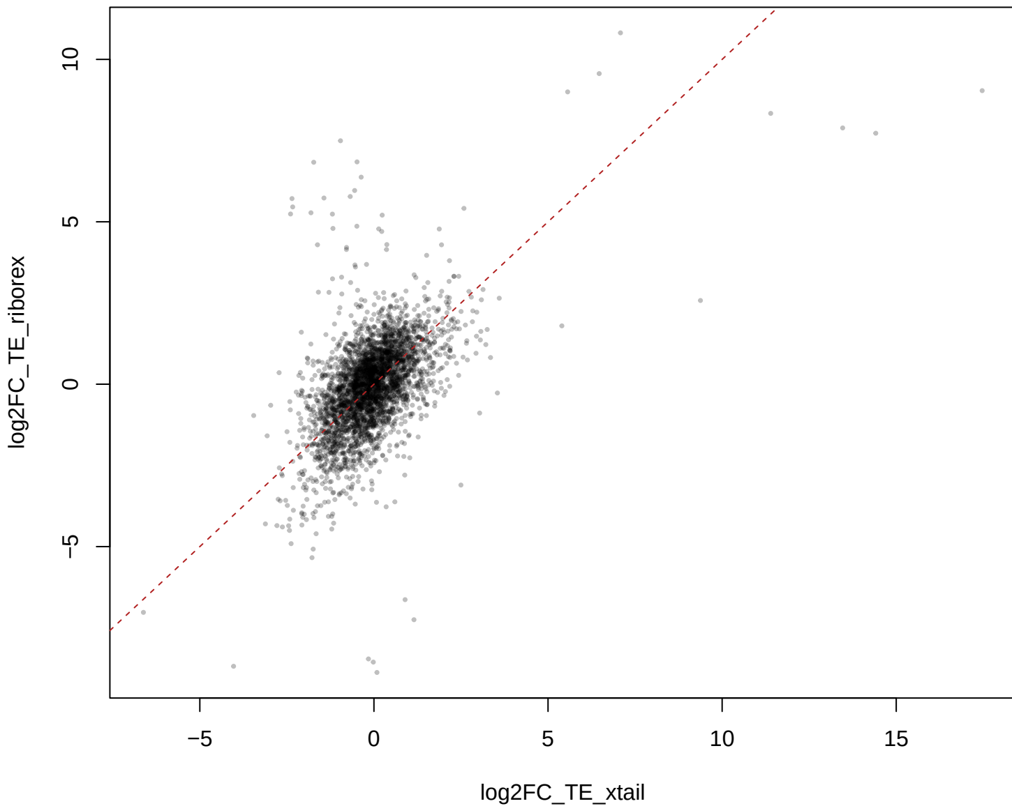
xtail vs riborex ( r = 0.543 )
