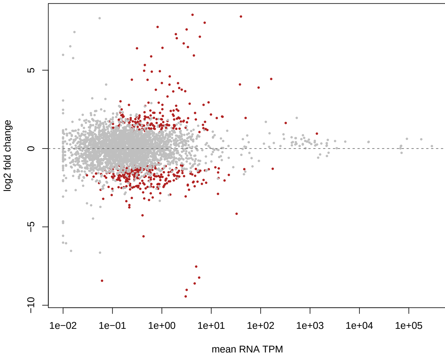
RNA log2FC vs expression
