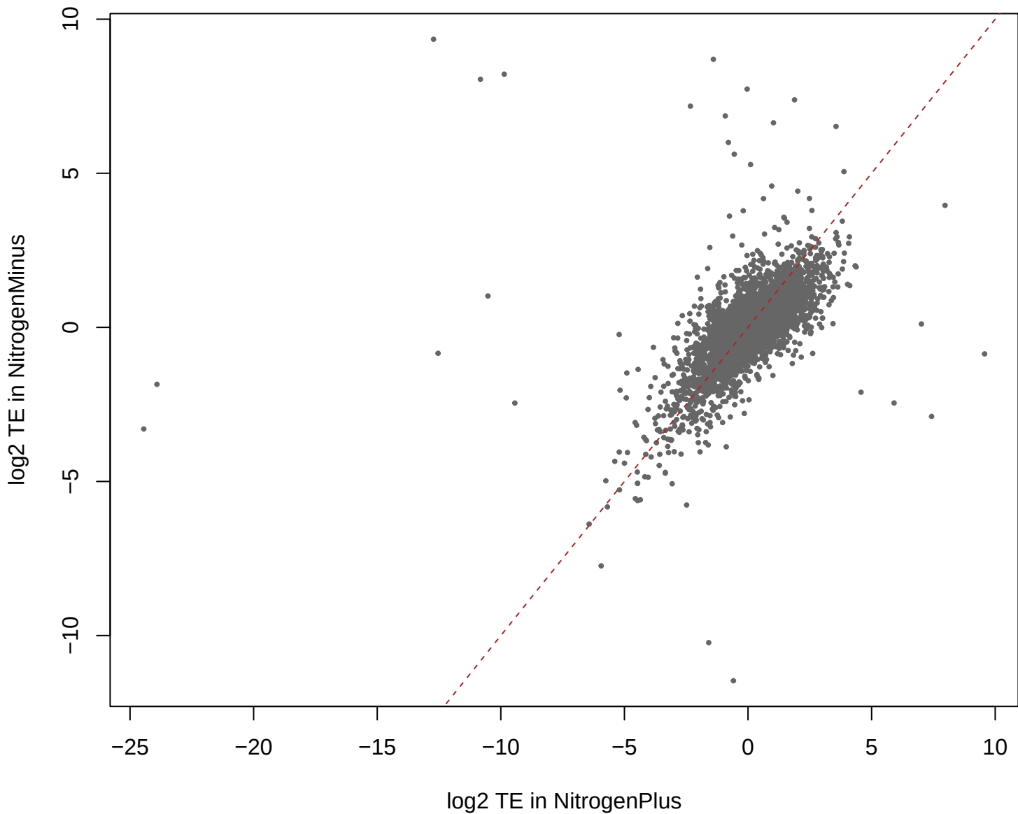
Within-condition log2 TE (xtail)
