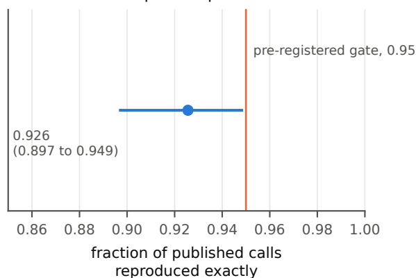
c The gate n = 1465 calls, 129 species; interval: bootstrap over species
