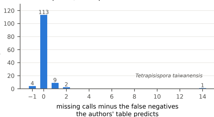
b Misses against the authors' prediction n = 129 species; unit: species
