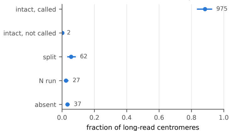
b Where each long-read centromere is n = 1103 centromeres in 69 strains; interval over strains
