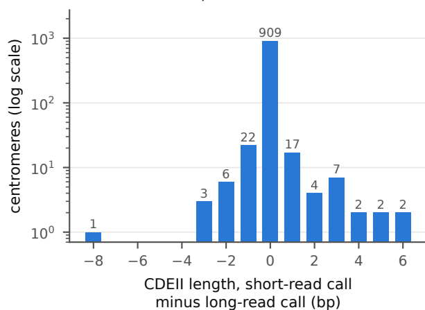
c CDEII length, 909 of 975 identical unit: centromere, 69 strains
