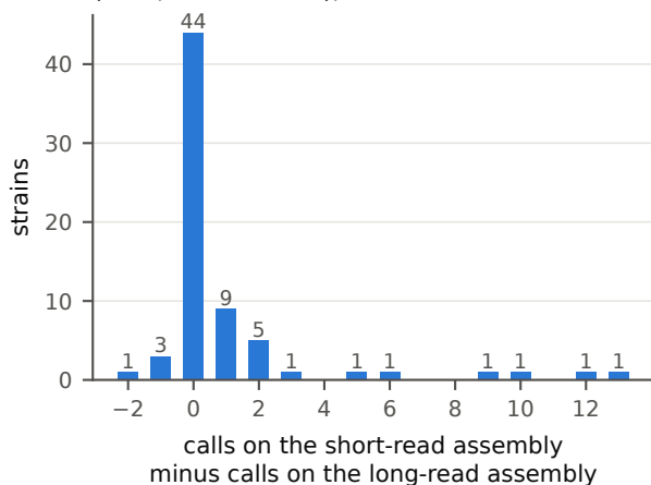
a Call counts, 44 of 69 strains equal (0.64, 0.52 to 0.74); unit: strain
