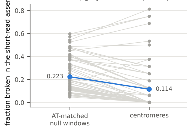
d Breaks: ratio 0.51 (0.35 to 0.66), Holm p 0.0013 n = 69 strains; grey: each strain; blue: pooled
