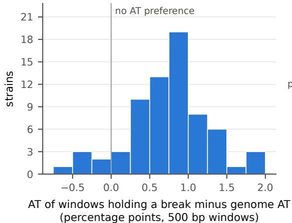
a Published short-read assemblies (arm 2) n = 69 strains, 63 above zero; unit: strain
