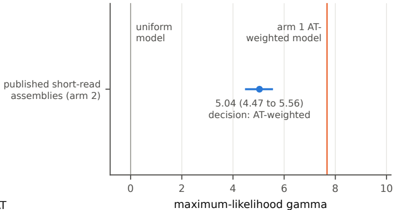
b Which breakpoint model fits interval: bootstrap over strains
