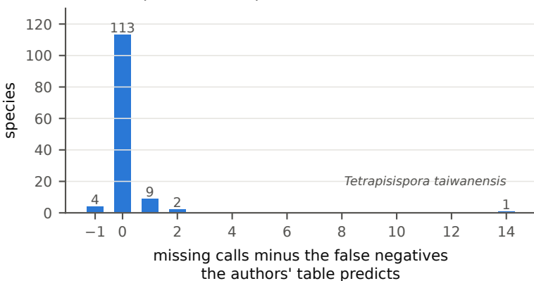
b Misses against the authors' prediction n = 129 species; unit: species
