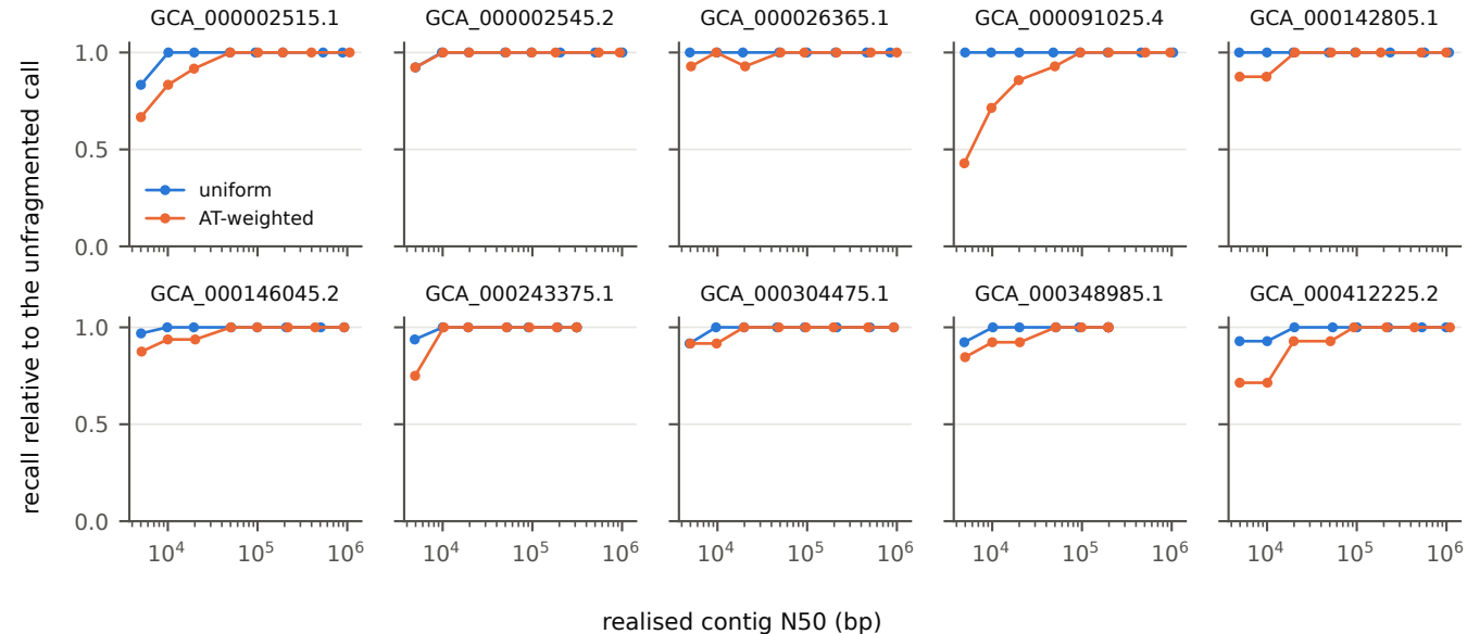
Simulation: recall per genome, median of 10 replicates per level; unit: genome
