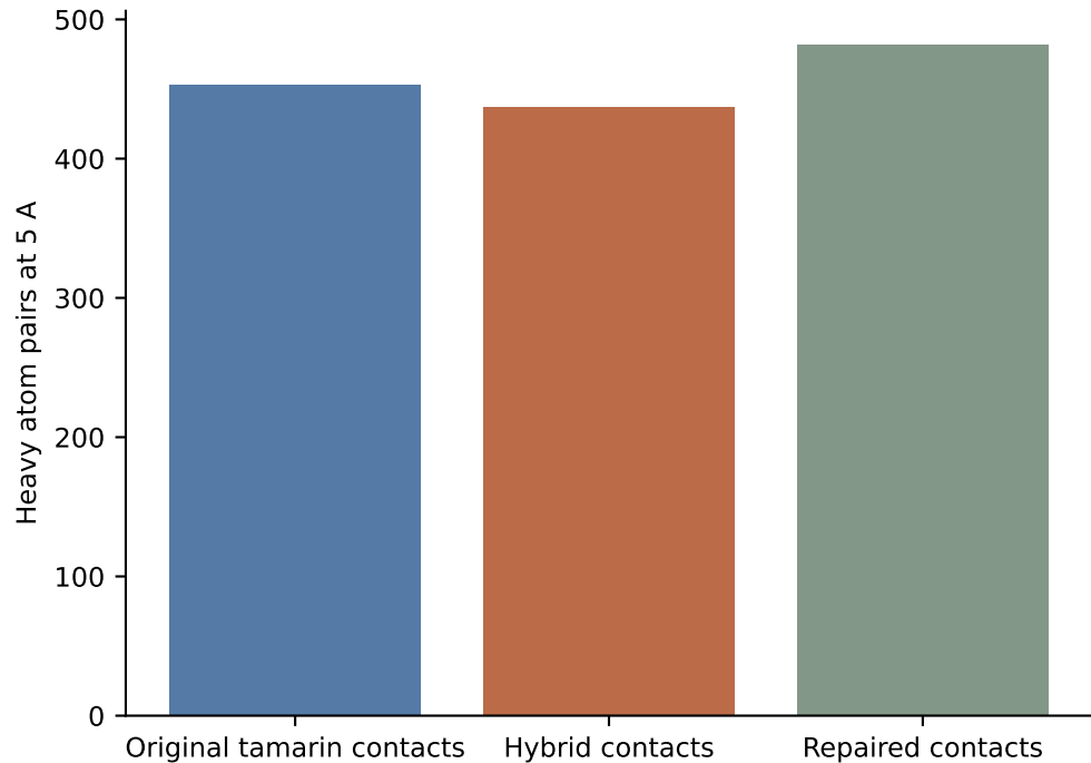
CA RMSD 3.69 Å; initial clashes 10
