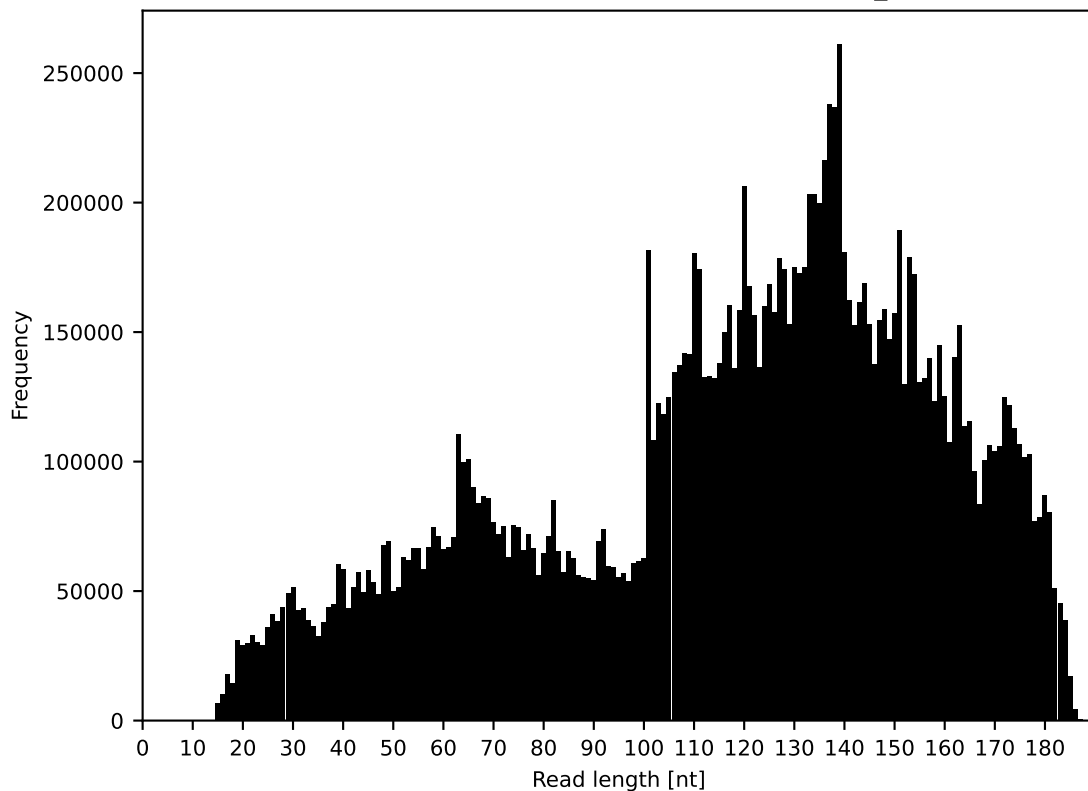
Length distribution of the input reads - salt_r1
