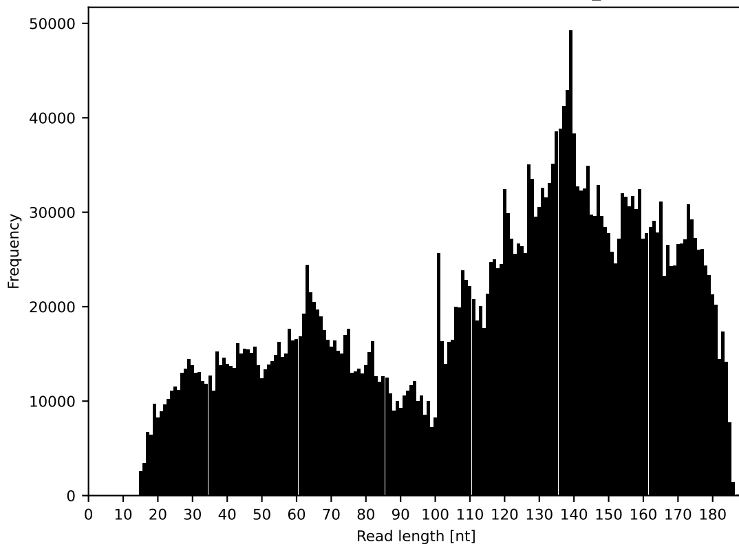
Length distribution of the input reads - salt_r2
