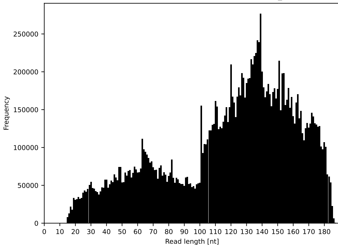
Length distribution of the input reads - control_r1
