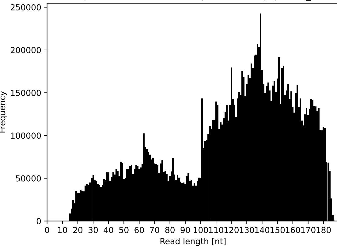
Length distribution of the input reads - apigennin_r1
