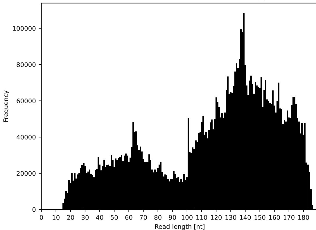
Length distribution of the input reads - control_r2
