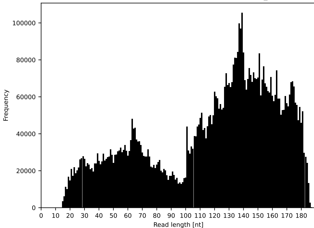
Length distribution of the input reads - apigennin_r2
