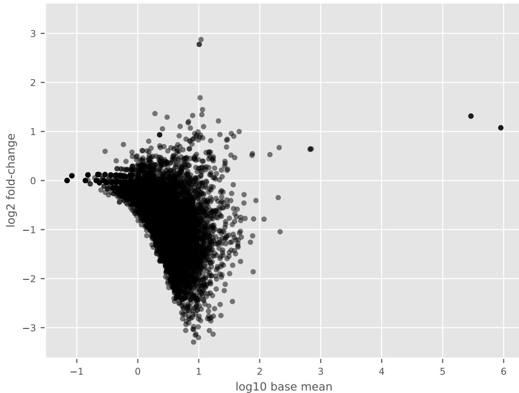
salt vs. apigennin - MA plot
