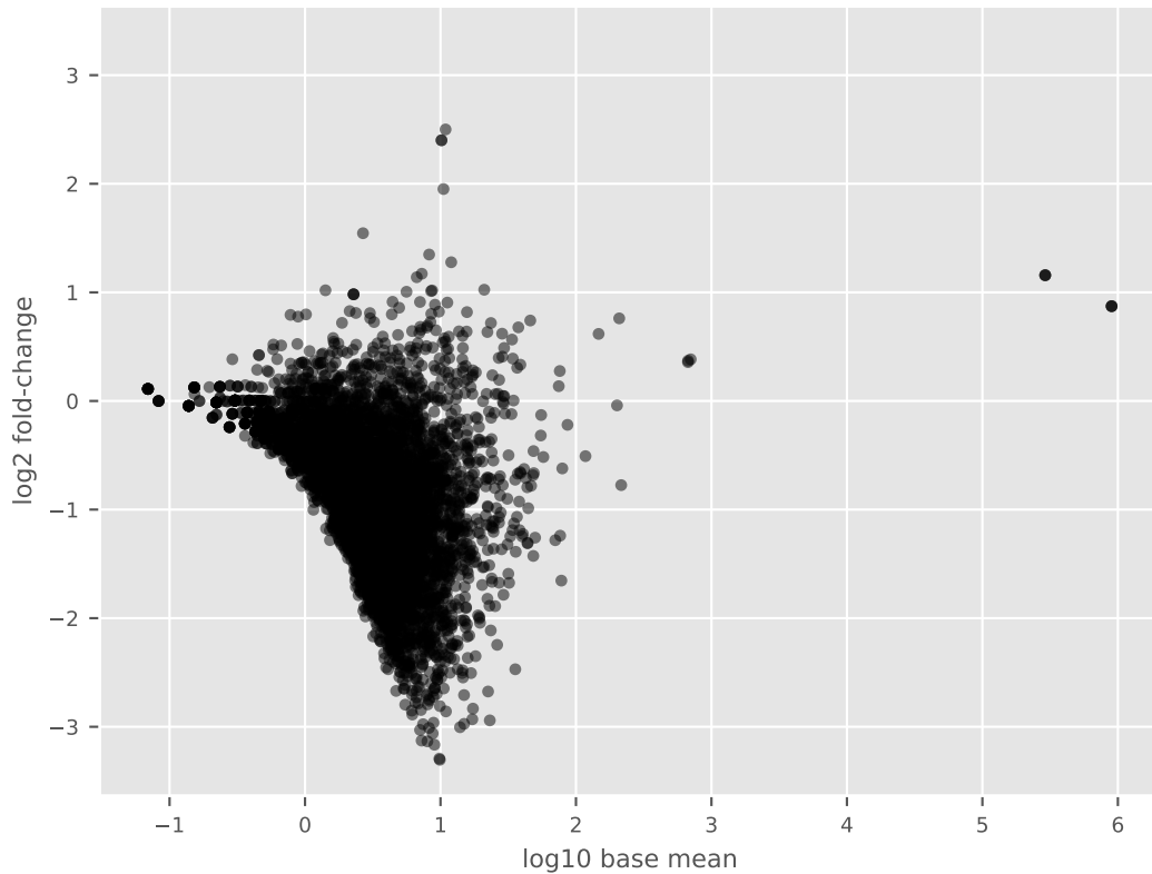
salt vs. control - MA plot
