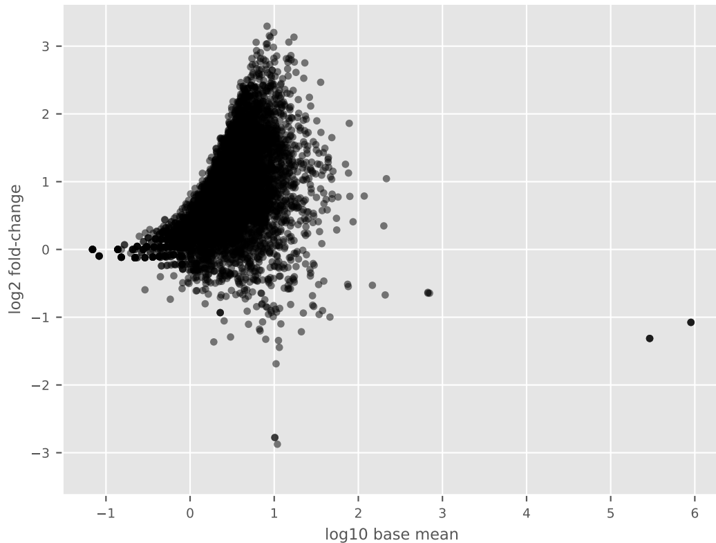
apigennin vs. salt - MA plot
