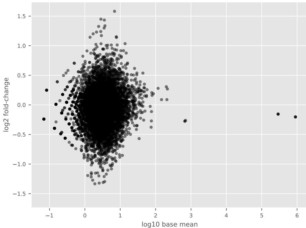
apigennin vs. control - MA plot
