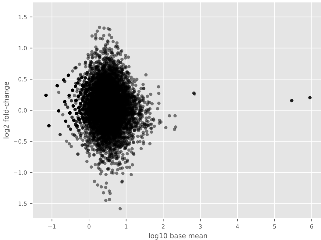
control vs. apigennin - MA plot
