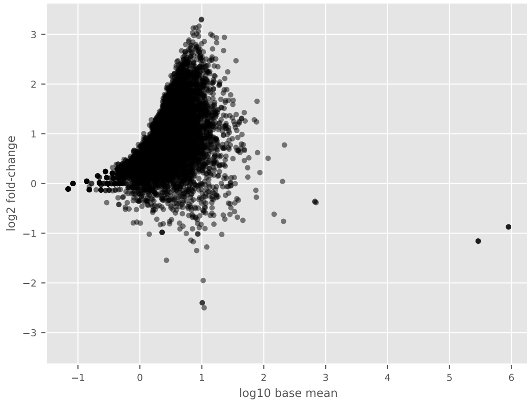
control vs. salt - MA plot
