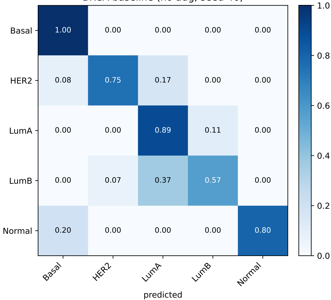
BRCA baseline (no aug, seed 46)
