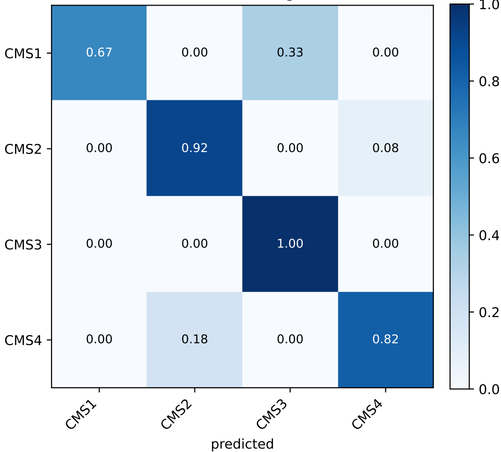
COAD baseline (no aug, seed 42)
