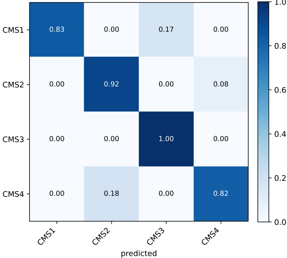
COAD baseline (no aug, seed 44)
