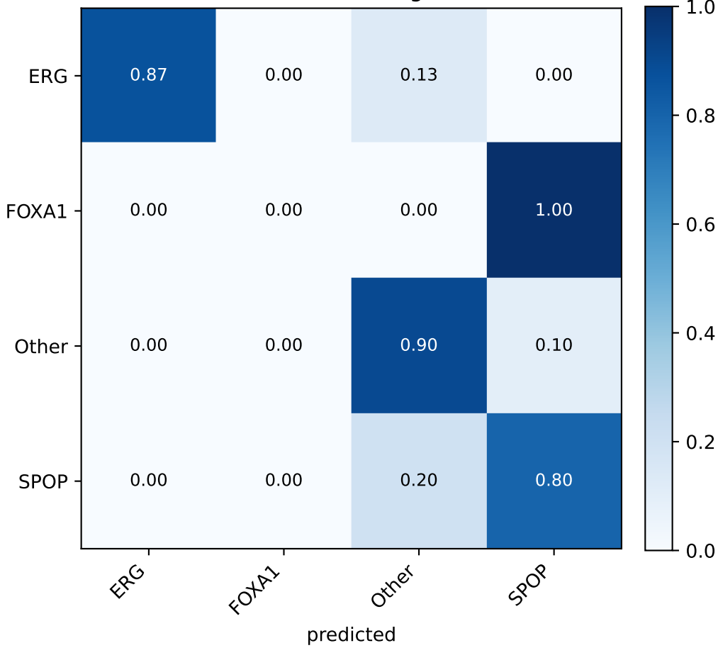
PRAD baseline (no aug, seed 46)
