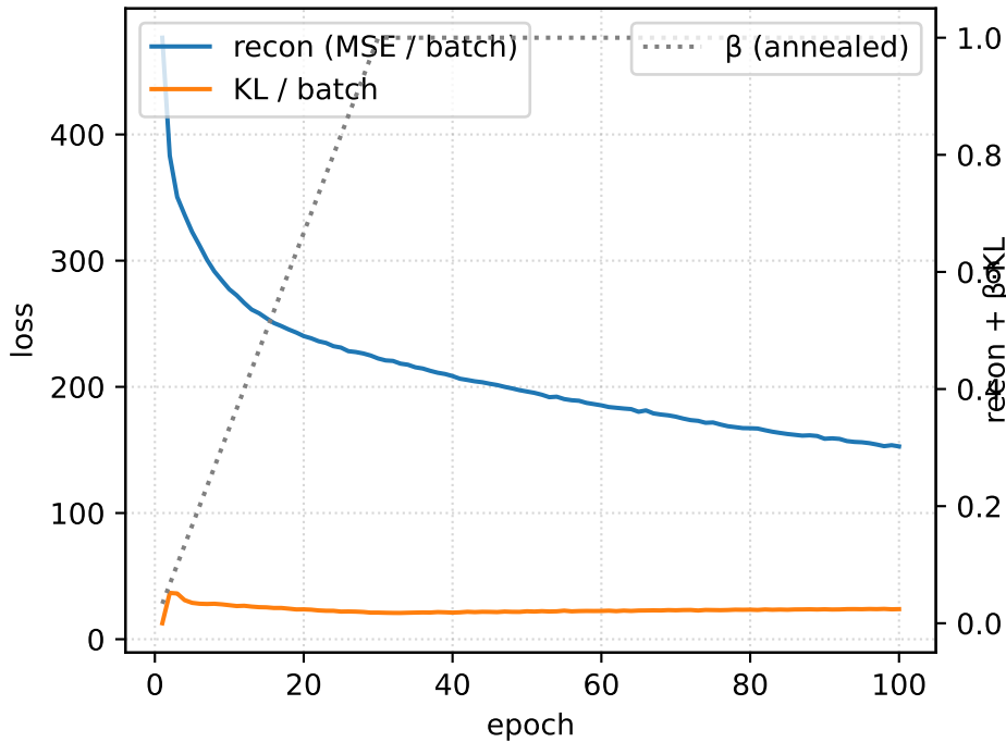
BRCA cVAE training (recon + KL + \beta )
