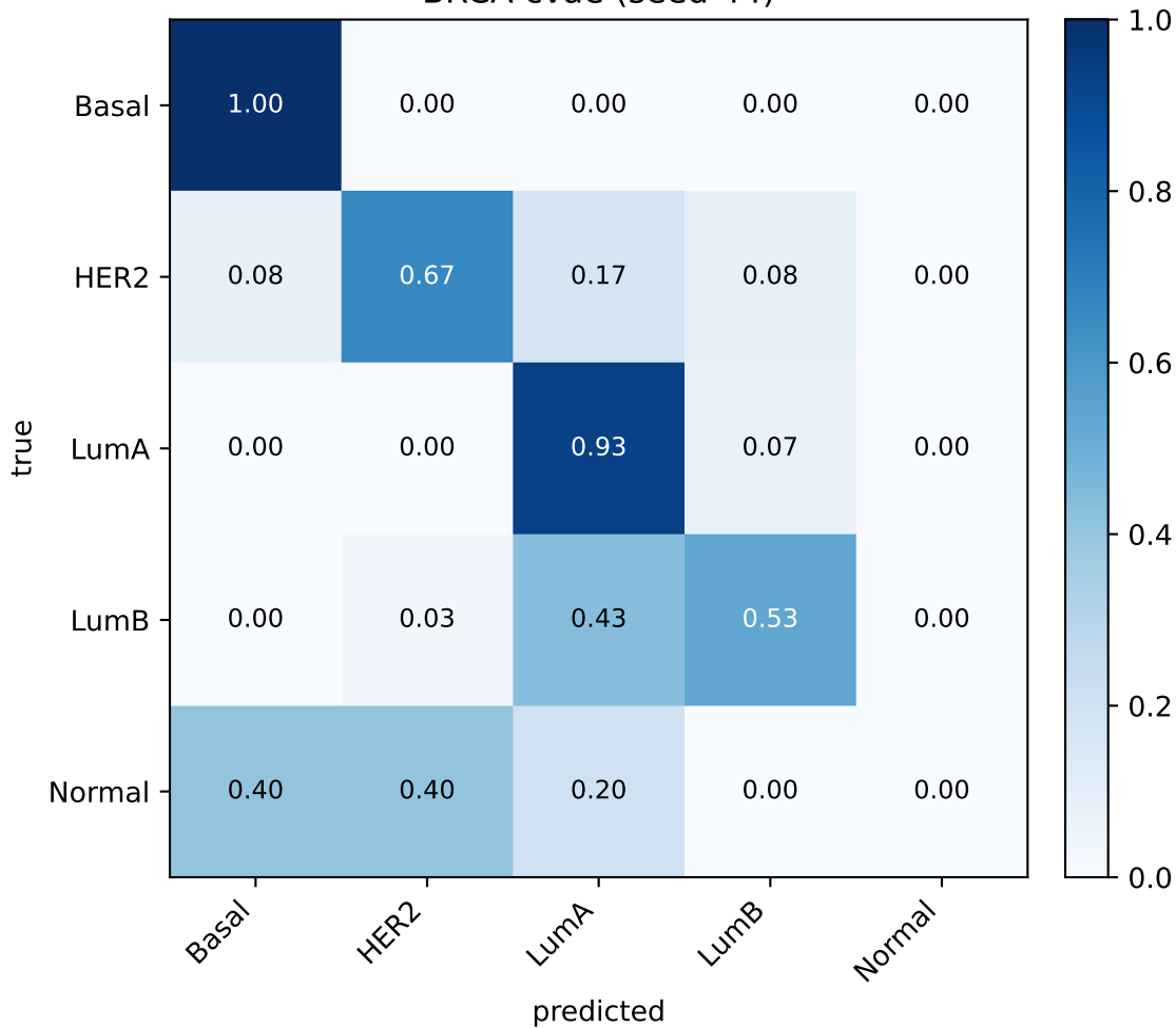
BRCA cvae (seed 44)
