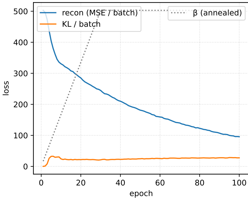
COAD cVAE training (recon + KL + \beta )
