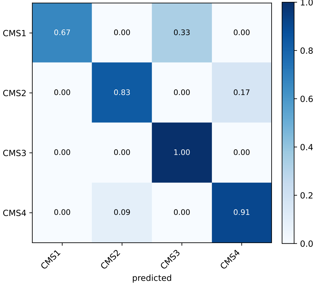
COAD cvae (seed 42)
