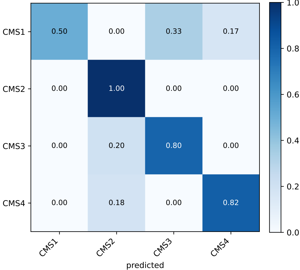
COAD cvae (seed 43)
