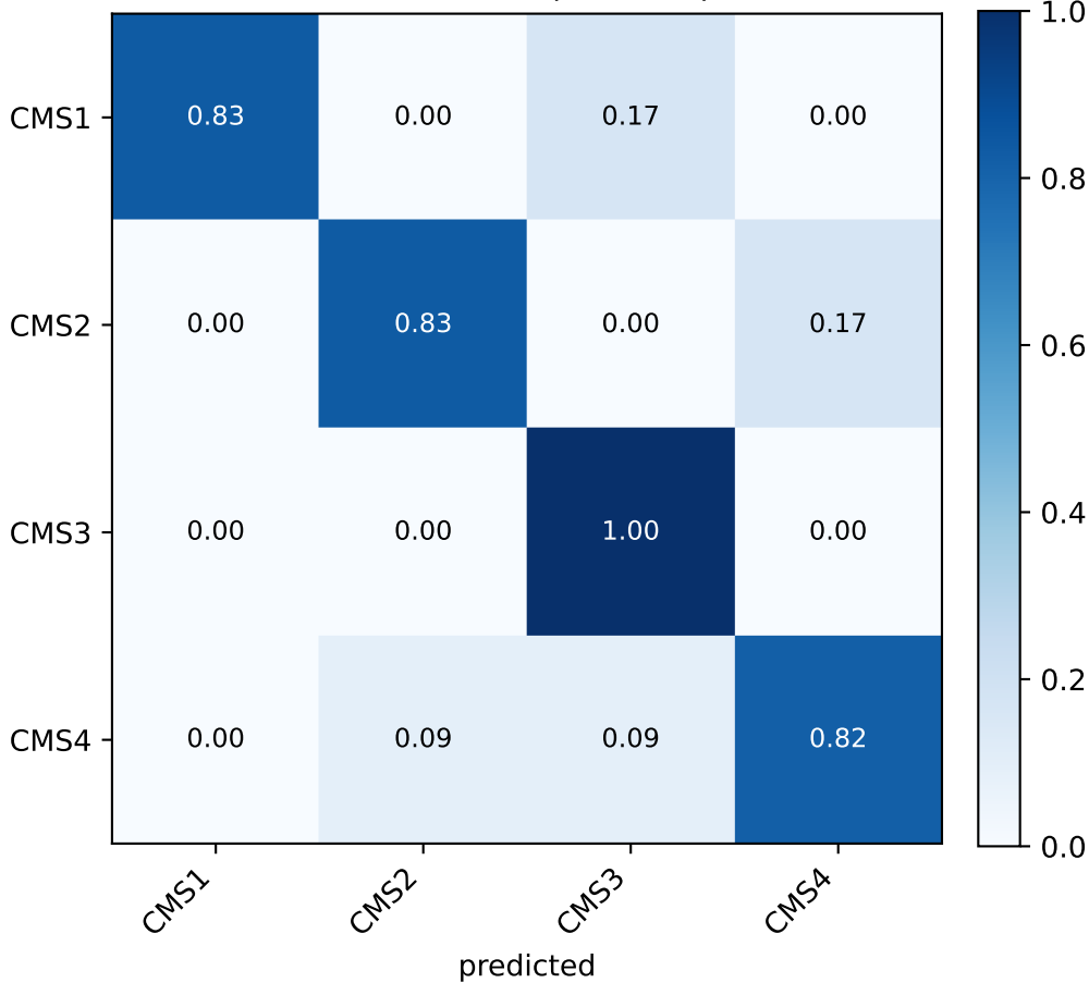
COAD cvae (seed 44)
