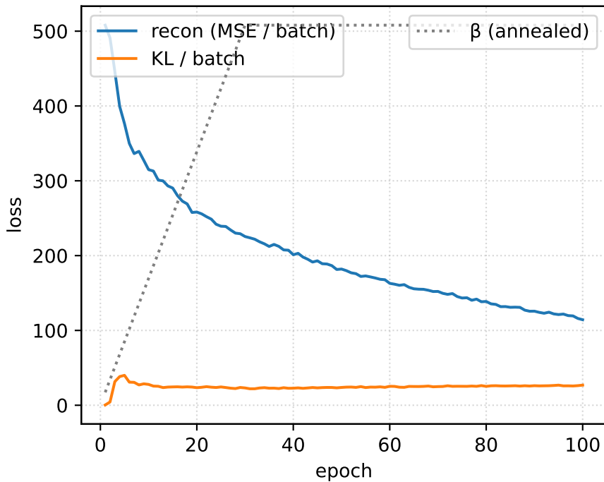
PRAD cVAE training (recon + KL + \beta )
