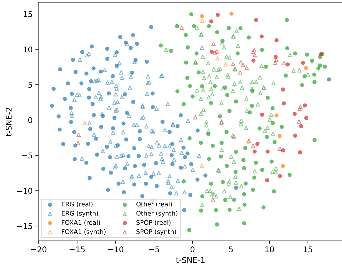
PRAD t-SNE overlay (real train vs cVAE synthetic)
