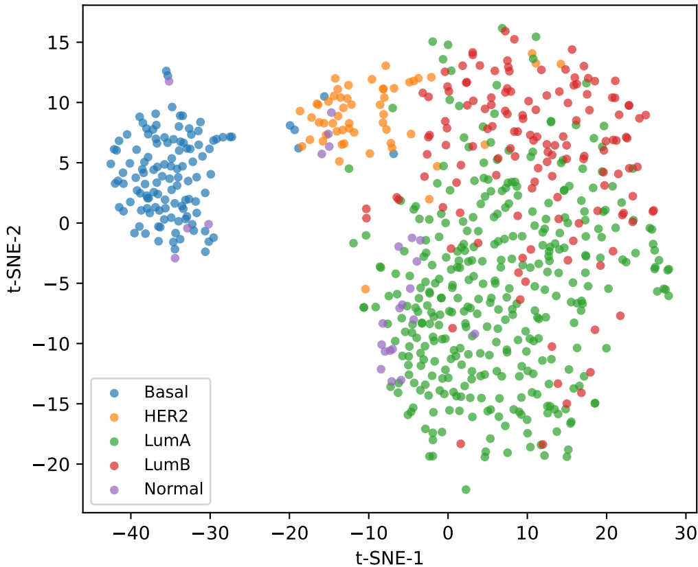
BRCA t-SNE of z-scored top-500 genes (train, perplexity=30)
