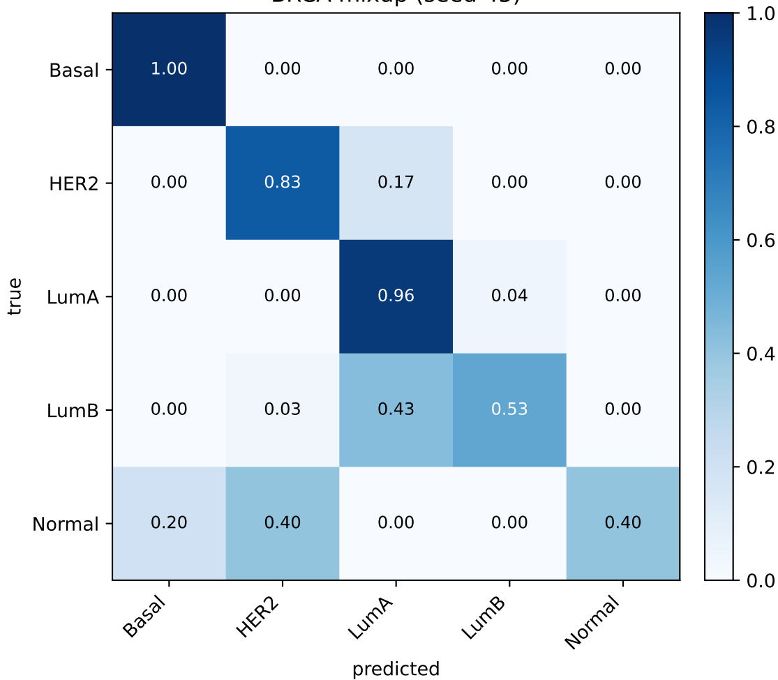
BRCA mixup (seed 45)
