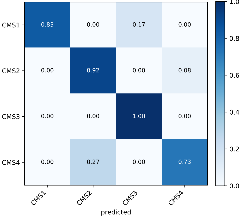
COAD mixup (seed 42)
