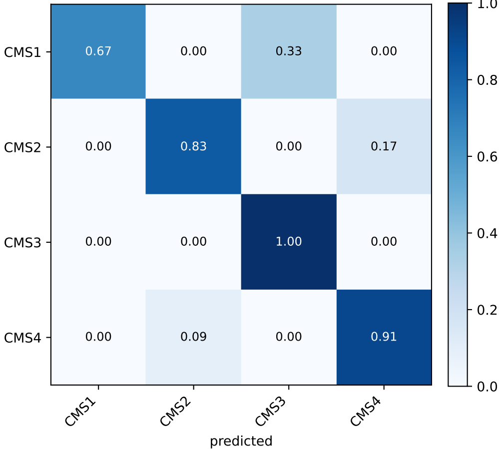
COAD mixup (seed 46)
