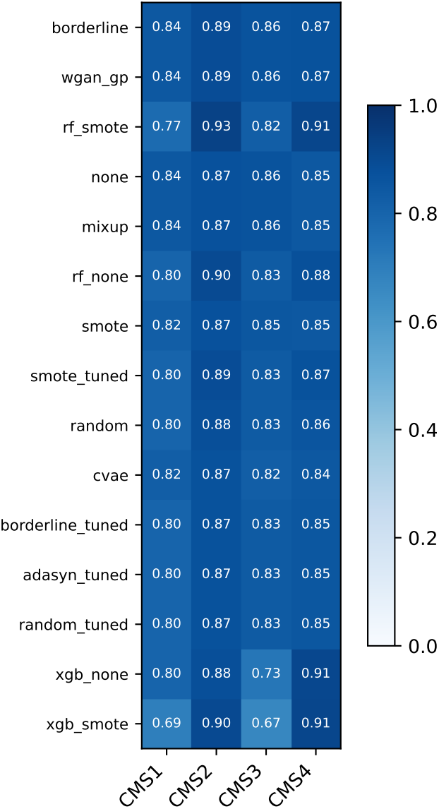
COAD per-class F1 (mean over seeds)
