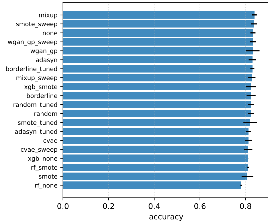
BRCA — accuracy (mean \pm std over seeds)
