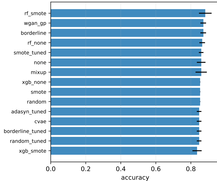
COAD — accuracy (mean \pm std over seeds)
