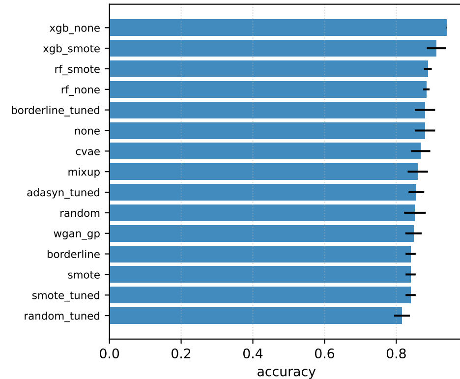
PRAD — accuracy (mean \pm std over seeds)
