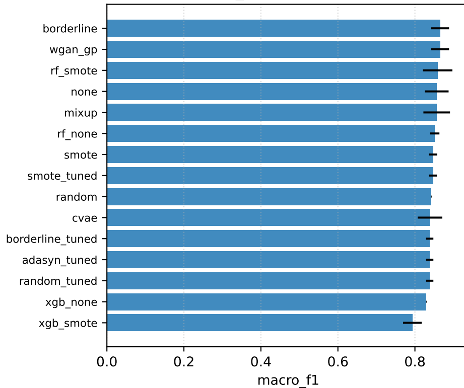
COAD — macro_f1 (mean \pm std over seeds)
