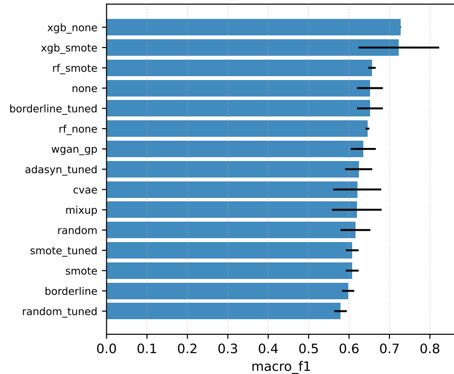
PRAD — macro_f1 (mean \pm std over seeds)
