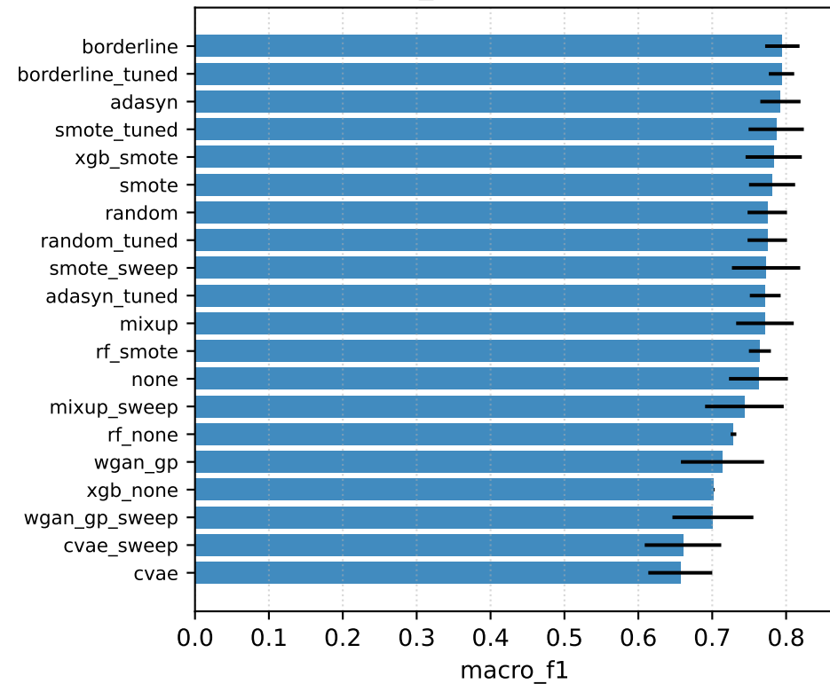
BRCA — macro_f1 (mean \pm std over seeds)
