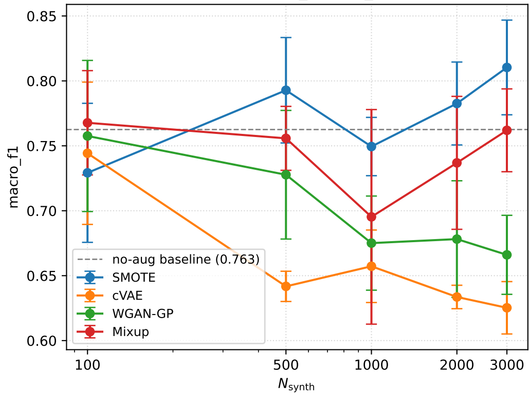
BRCA — macro_f1 vs N_{\text{synth}}
