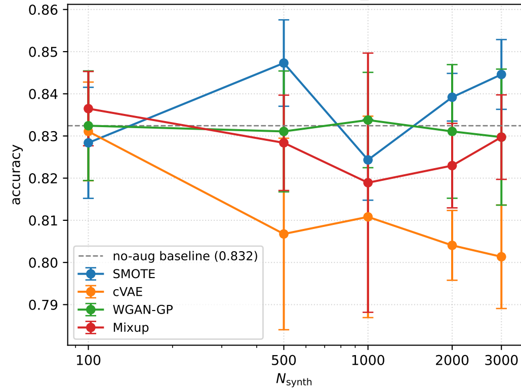
BRCA — accuracy vs N_{\text{synth}}
